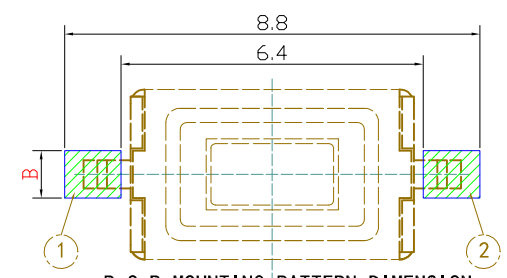
P. C. B MOUNTING PATTERN DIMENSION the following soldering are recommended for reflow soldering
